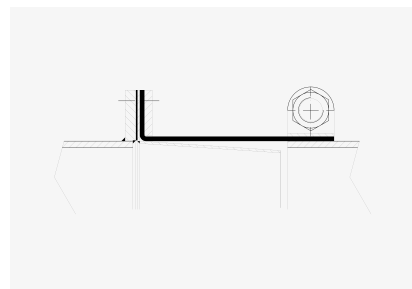
Cylindrical with inner sleeve, flange on one side, band clamp on other side
