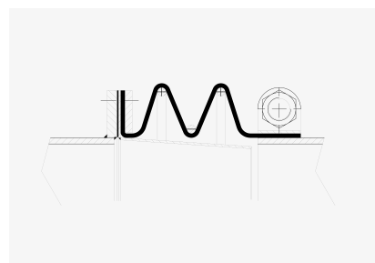
Double convolution with inner sleeve and vacuum support rings, flange on one side, band clamp on other side
