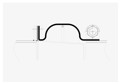
Single convolution with inner sleeve and vacuum support ring, flange on one side, band clamp on other side
