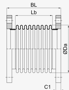
DN 50 - DN 80
