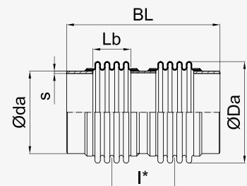
DN 100 - DN 2400
