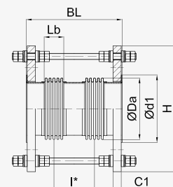
DN 100 - DN 400
