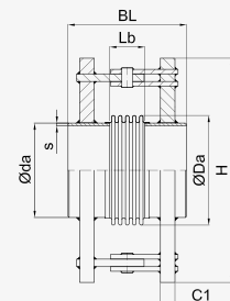
DN 100 - DN 800
