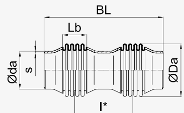
DN 50 - DN 80
