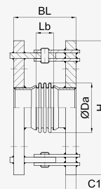
DN 50 - DN 80
