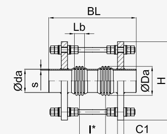
DN 50 - DN 80
