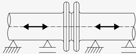
Absorption of axial expansion along the pipe axis using an axial expansion joint
