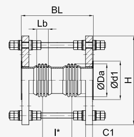
DN 50 - DN 80
