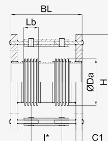
DN 50 - DN 80
