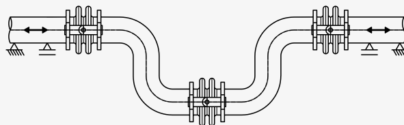
Axial expansions acting in a U-shaped arrangement are deflected in three angular movements (three hinges). This design is intended for absorbing large axial expansions in the pipe.
