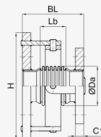
DN 50 - DN 80
