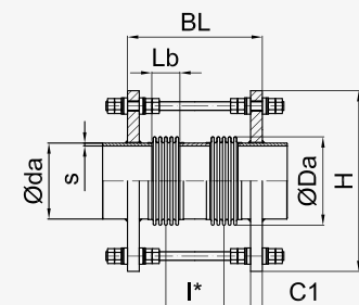
DN 100 - DN 1800
