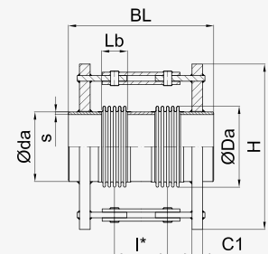
DN 50 - DN 80
