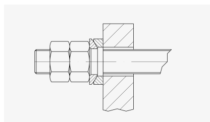
External tensioning (without negative pressure)
