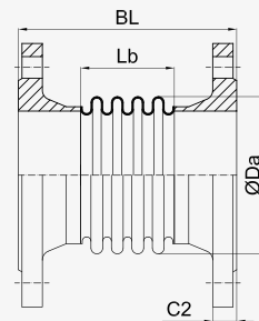
DN 50 - DN 80
