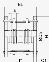
DN 50 - DN 80
