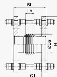
DN 50 - DN 80
