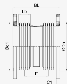
DN 100 - DN 1400
