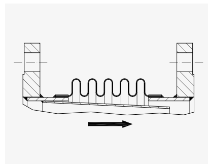
Lateral expansion joint with conical inner sleeve
