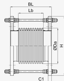
DN 50 - DN 80
