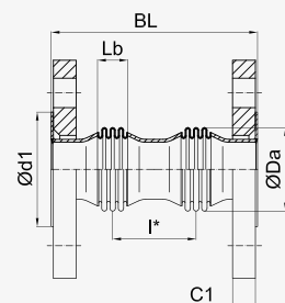
DN 50 - DN 80
