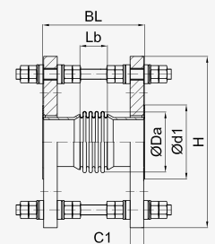
DN 50 - DN 80
