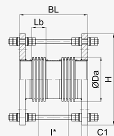
DN 100 - DN 800
