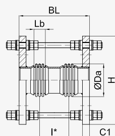
DN 50 - DN 80
