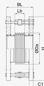
DN 100 - DN 800
