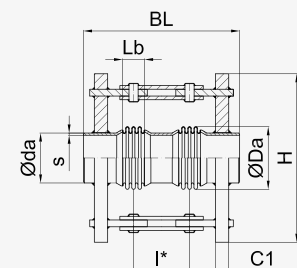
DN 50 - DN 80
