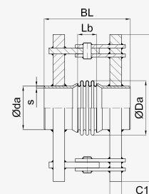
DN 50 - DN 80
